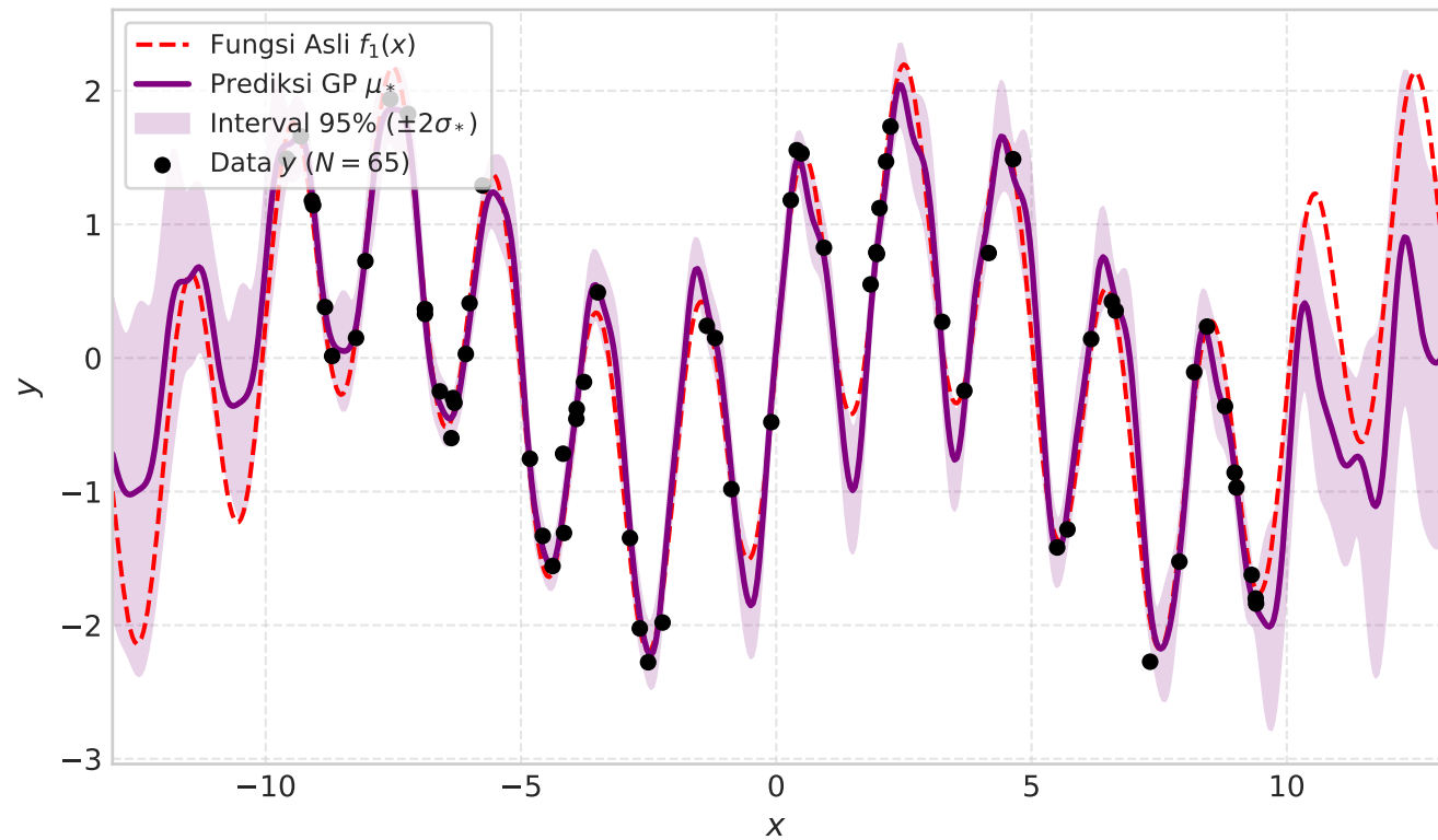
(b) Perkalian: k_{\text{RBF}} \times k_{\text{Per}}
